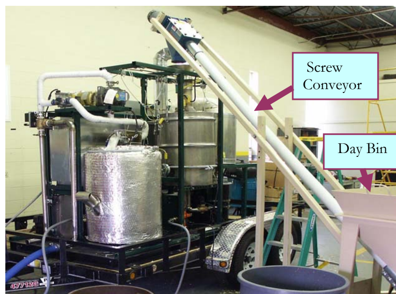
Photo 4-3: Screw Feeder of Gasifier System
