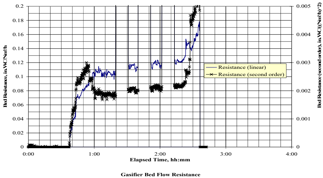
Figure B4: Gas Flow Resistance in Gasifier During a Typical Test Run
