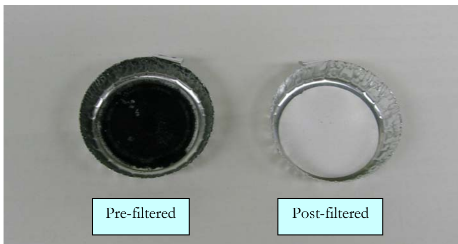
Photo 5-1: Comparisons of Pre- and Post-filtered Syn-gas Sampling Filter Papers
